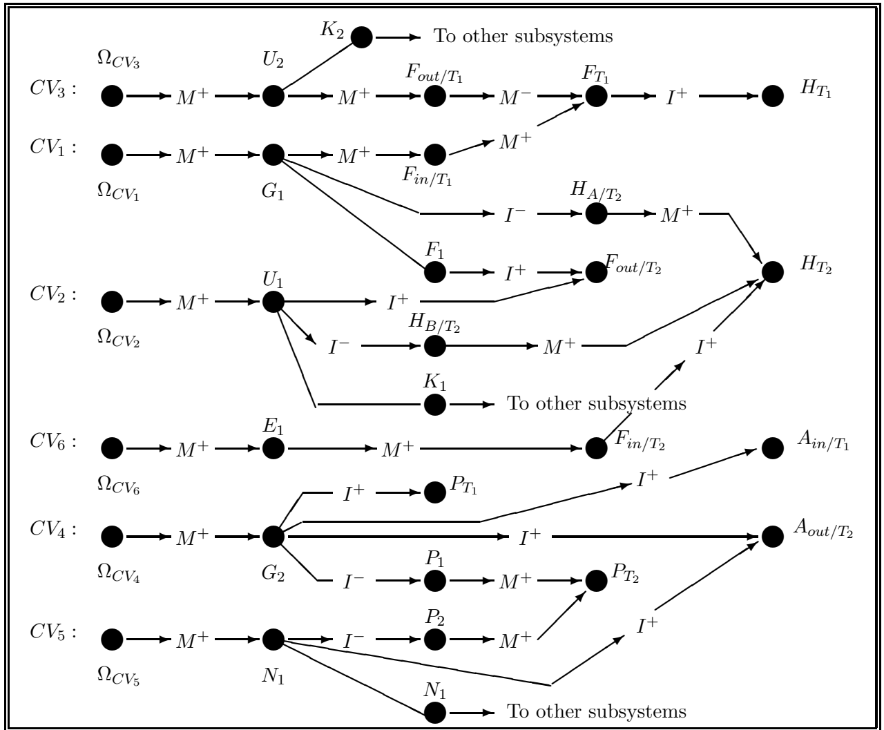
Figure 2.4: Qualitative flow graph for the pressure tank system.
