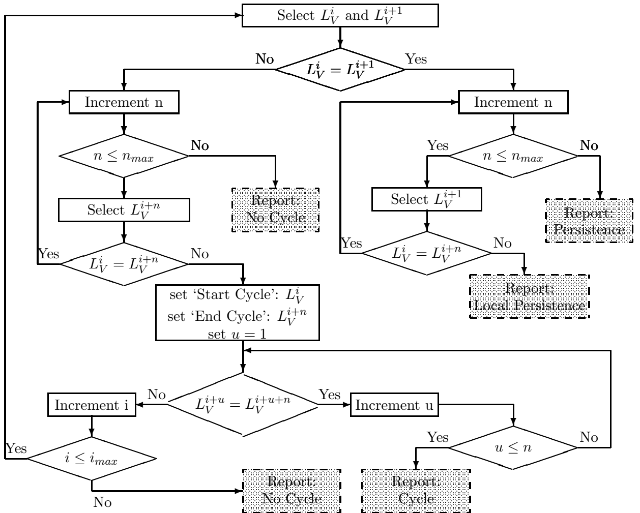
Figure 5.6: Repetition cycle detection algorithm.
