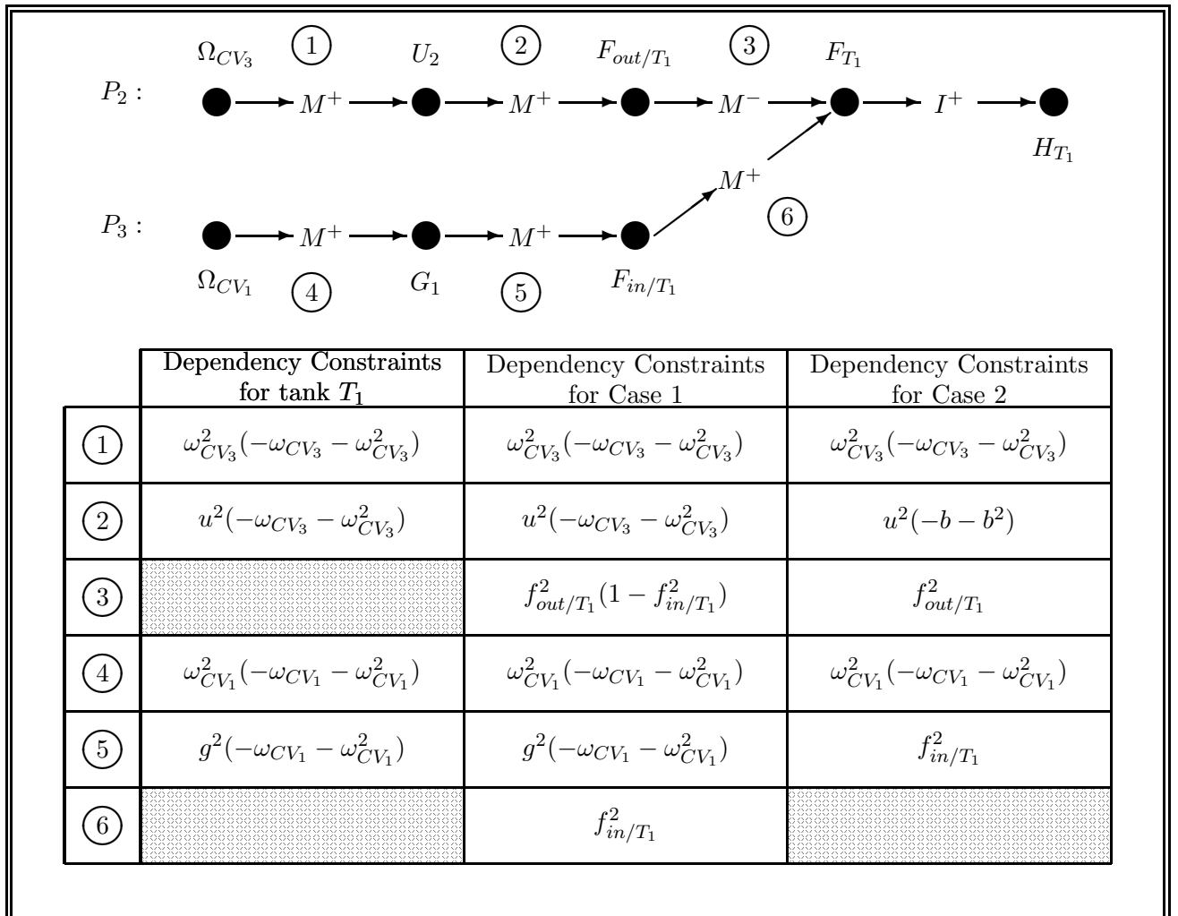
Figure 5.7: Qualitative model of the three design preferences for the tank T_1 .
