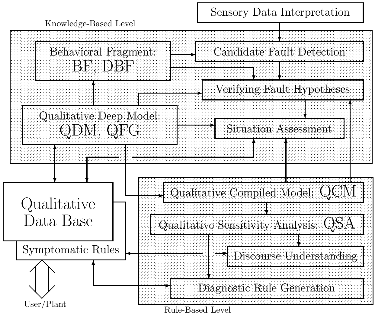
Figure 4.4: Subjective qualitative fault diagnosis system.
