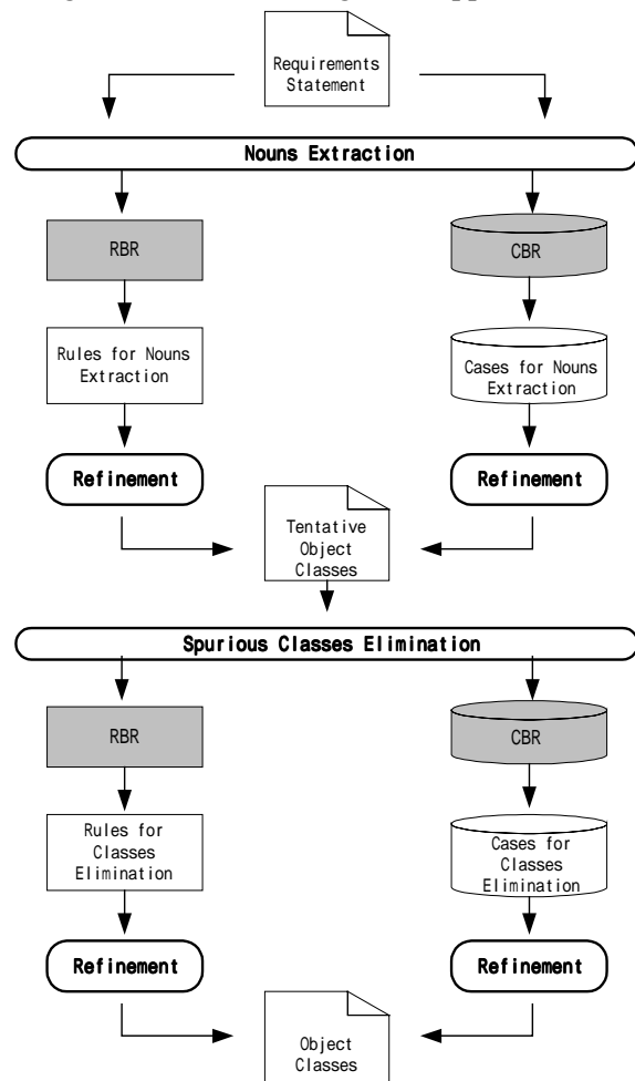
Figure 1: Architecture of the Object Classes' Identification in OOExpert
