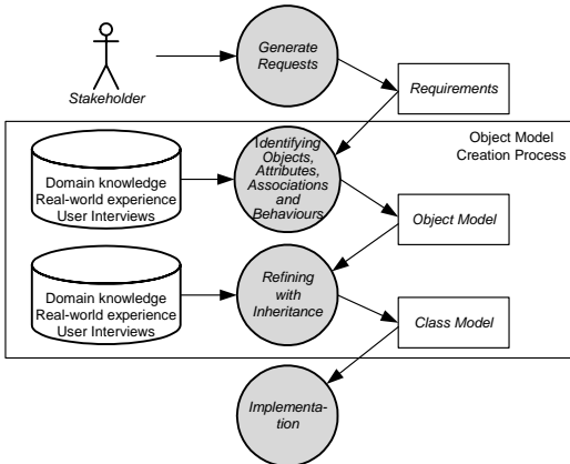
Fig. 1. Object Model Creation Process (OMCP).
