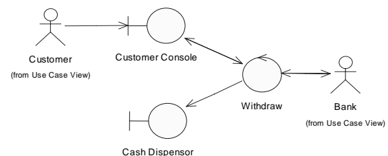
Fig. 3. Robustness diagram for withdraw cash.
