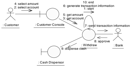
Fig. 4. Collaboration diagram for withdraw cash.
