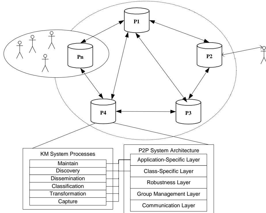
Figure 4. Typical structure of distributed peer to peer knowledge management systems.
